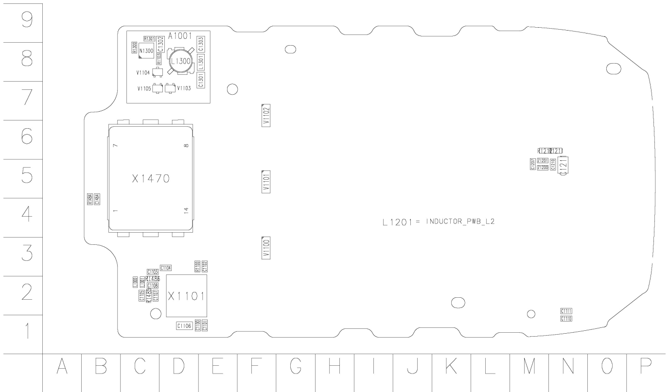
Figure 5 Component layout - top (1lha_50a)
